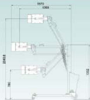
M-type stand dual gas cylinders
